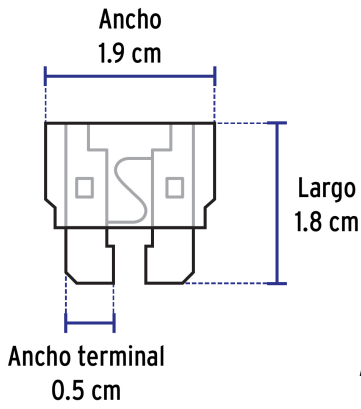
Fusible standard
